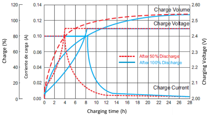
Charging curves Temperature 25°C (77°F)
