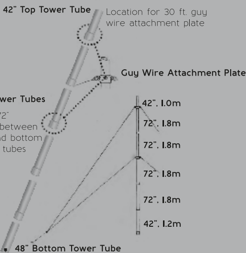
WINDFORCE™ -TOWER – XUNZEL Complete 8.8-meters Tower KIT for Wind Generators
